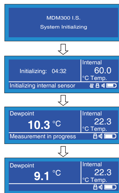
Figure 10 Start-Up Sequence
