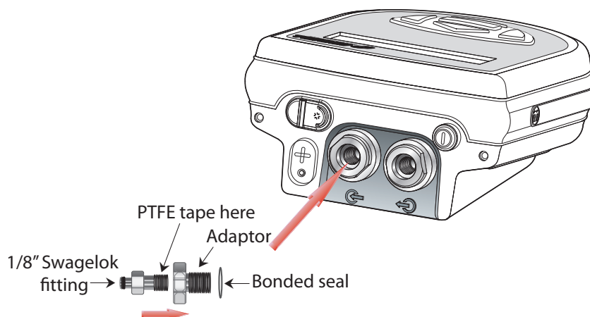
Figure 7 Bonded Seal Fitting
